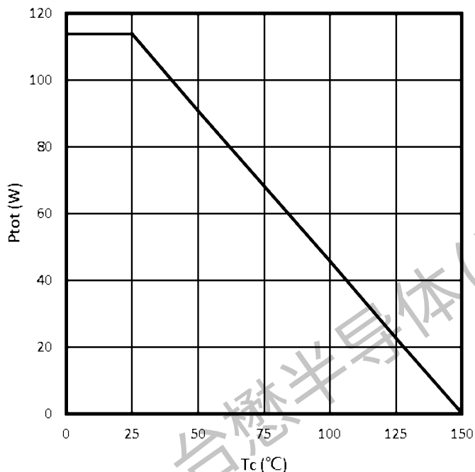
Power Dissipation
